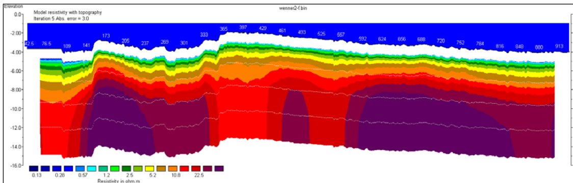
Interpreted marine resistivity section
