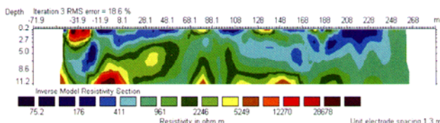
OhmMapper TR data collected over granite with surface weathering. Inversion done with RES2DINV program from MH lake
